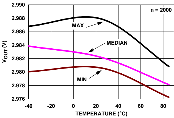
FIGURE 42. V OUT HIGH vs TEMPERATURE V S = ±1.5V, R L = 1k
