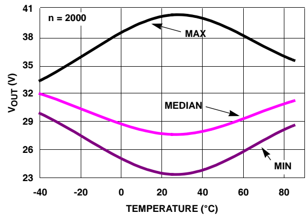
FIGURE 43. V OUT LOW vs TEMPERATURE V S = ±1.5V, R L = 1k
